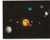
solar system
